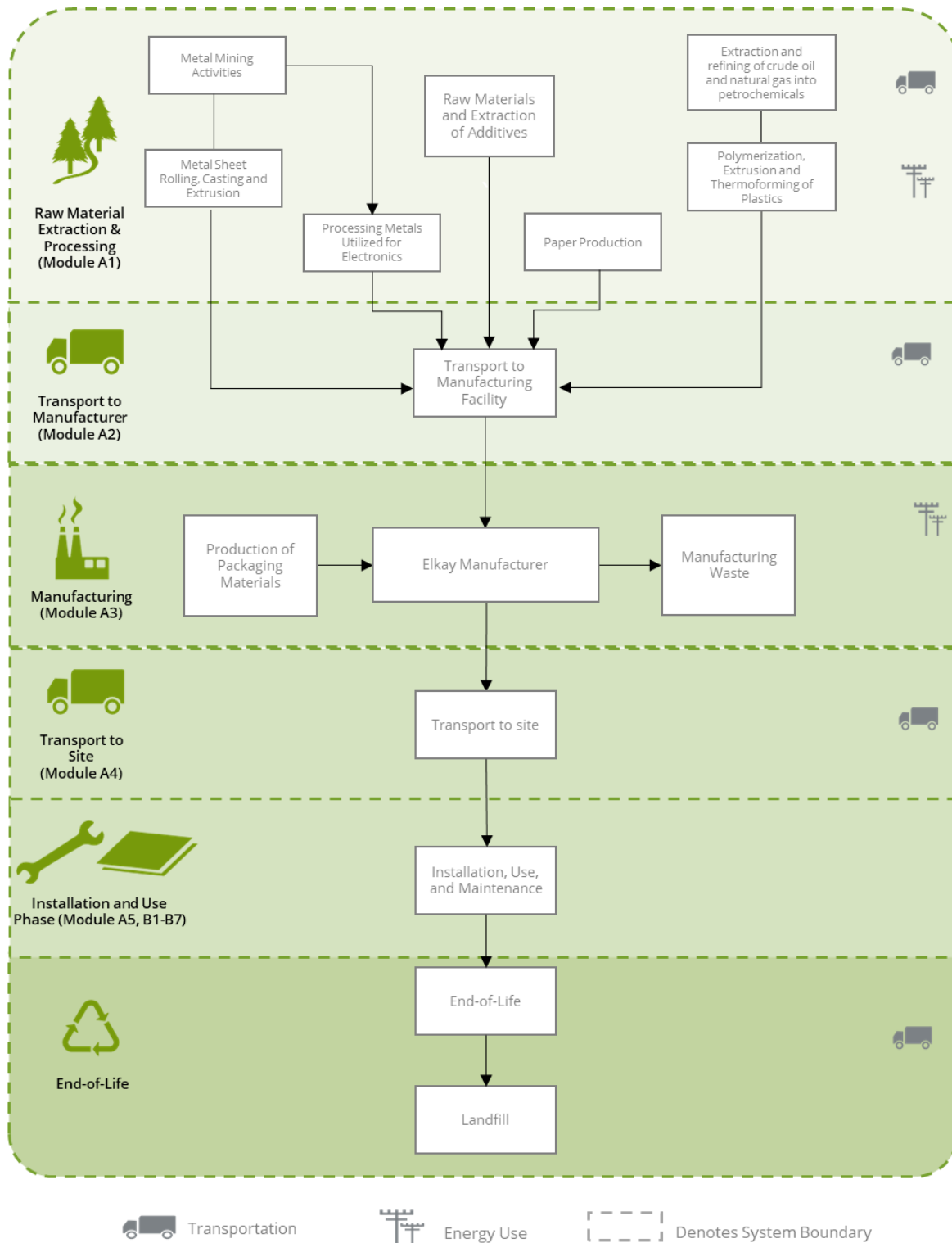
Figure 1. Flow diagram and system boundaries for the Elkay Enhanced Single Bottle Filling Station.
