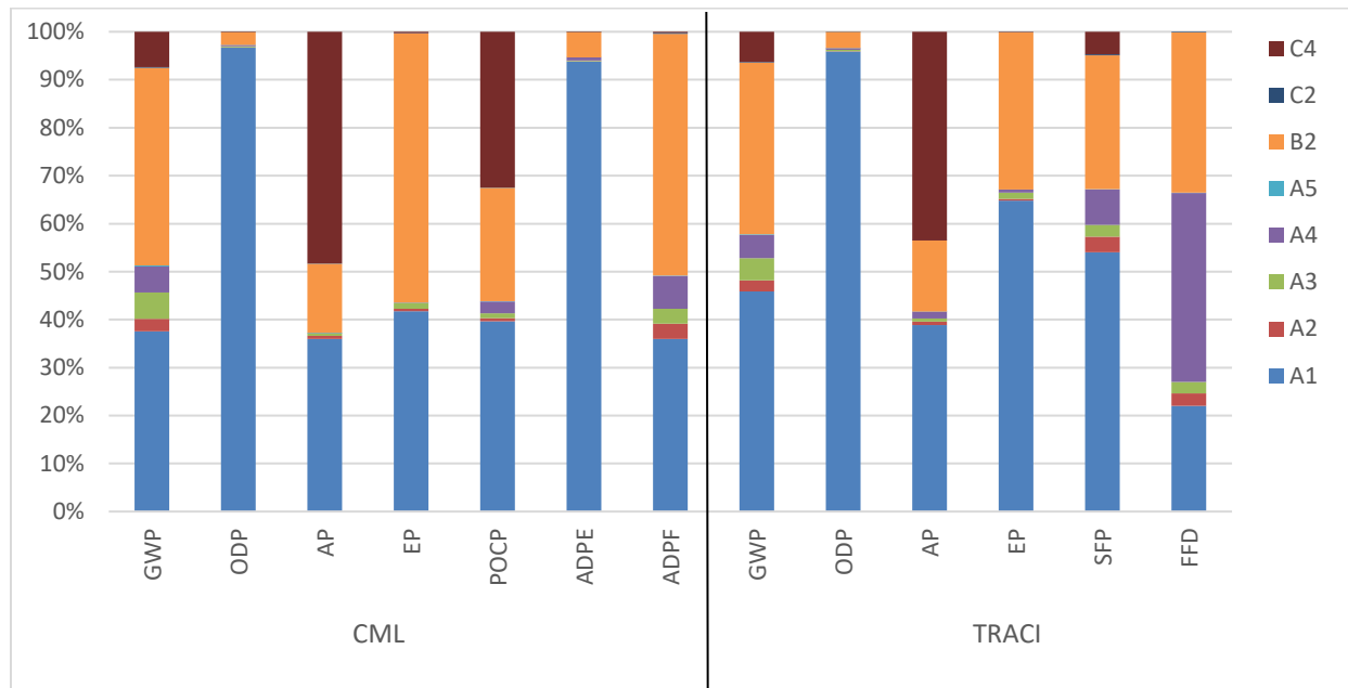
Figure 2. Contribution analysis for the Elkay Liv (LBWDC00 – N. America Model) Bottle Filling Stations (without Modules B4, B6, and B7).
